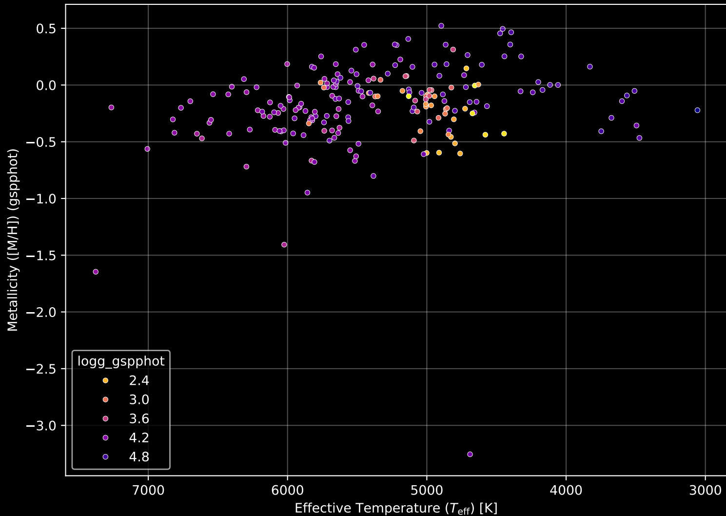
APOGEE DR17 Field: [086+47_MGA] Stellar Population Parameters (n= 205)
