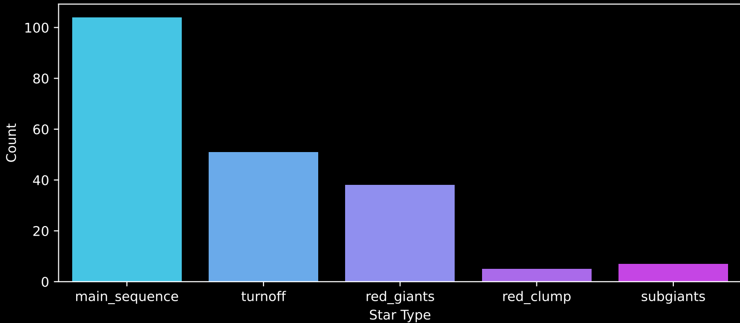
APOGEE DR17 Field: [086+47_MGA] Count plot of Star Type
