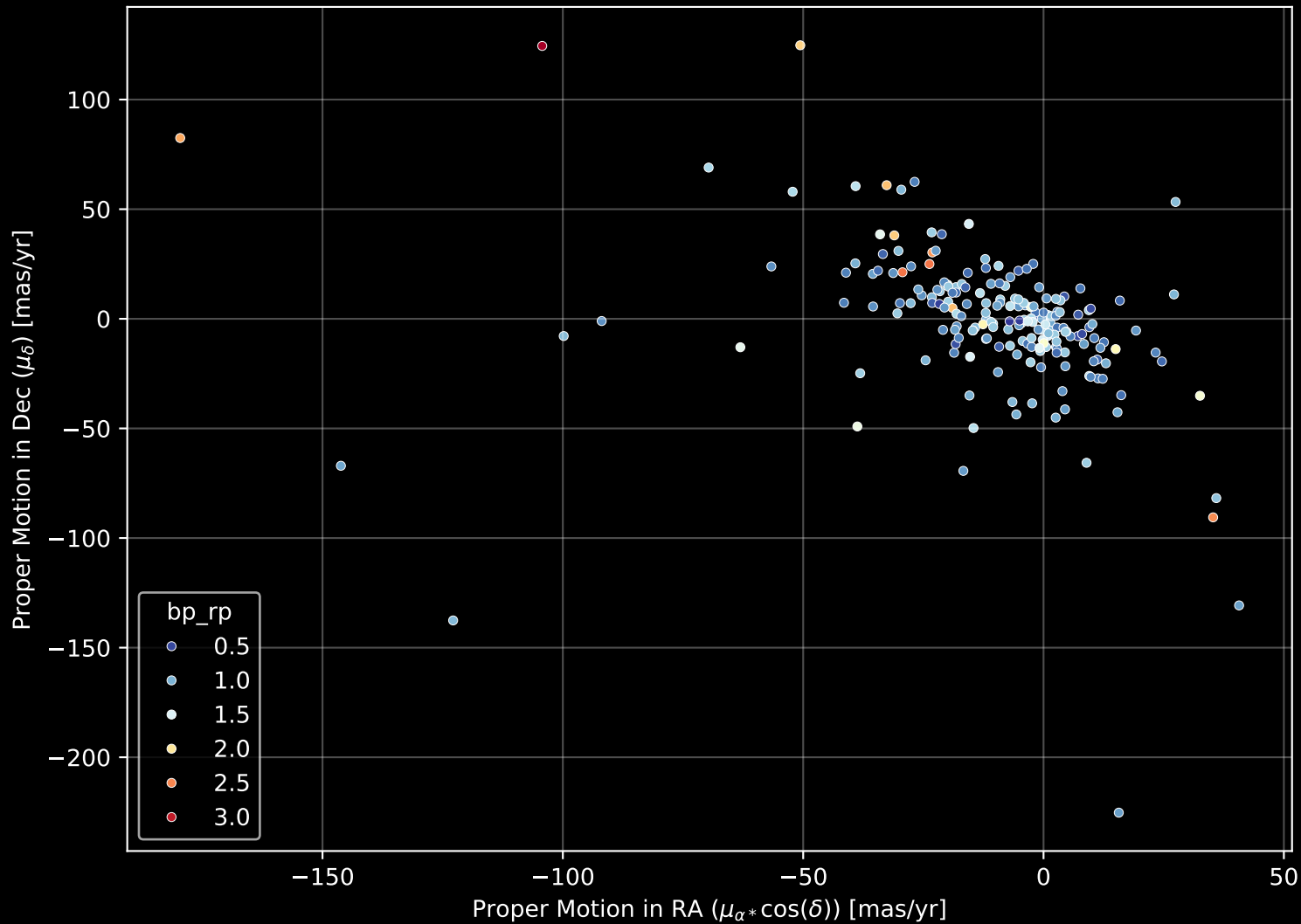
APOGEE DR17 Field: [086+47_MGA] Proper Motion Diagram (n= 205)
