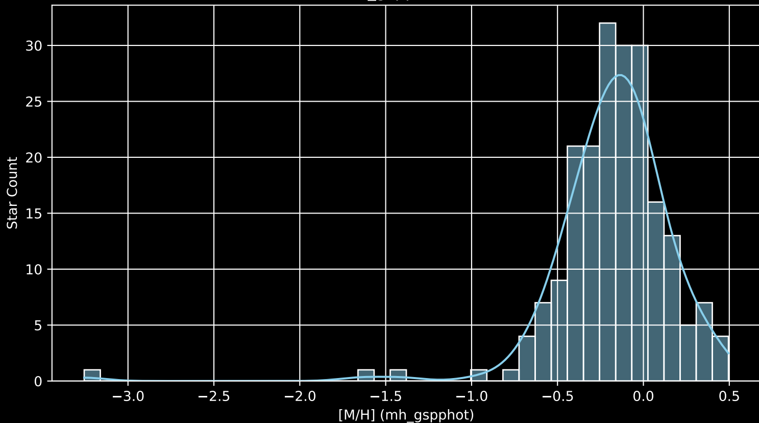
APOGEE DR17 Field: [086+47_MGA [M/H] (mh_gspphot) (n= 204)
