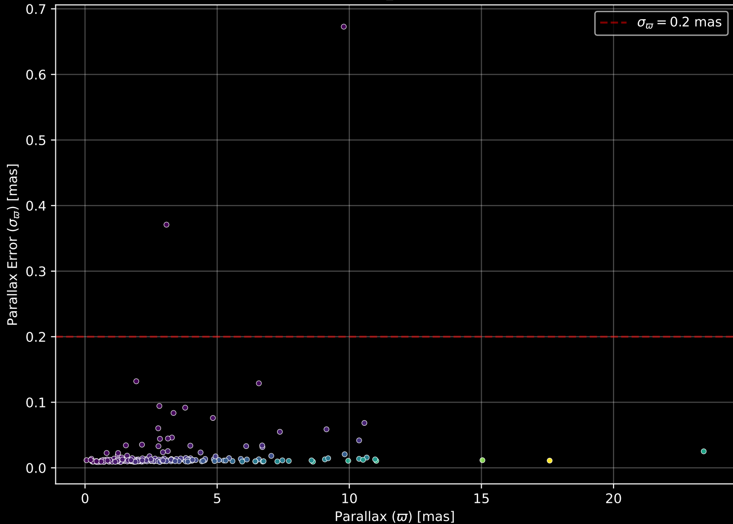
APOGEE DR17 Field: [086+47_MGA] Parallax Quality (n= 205)
