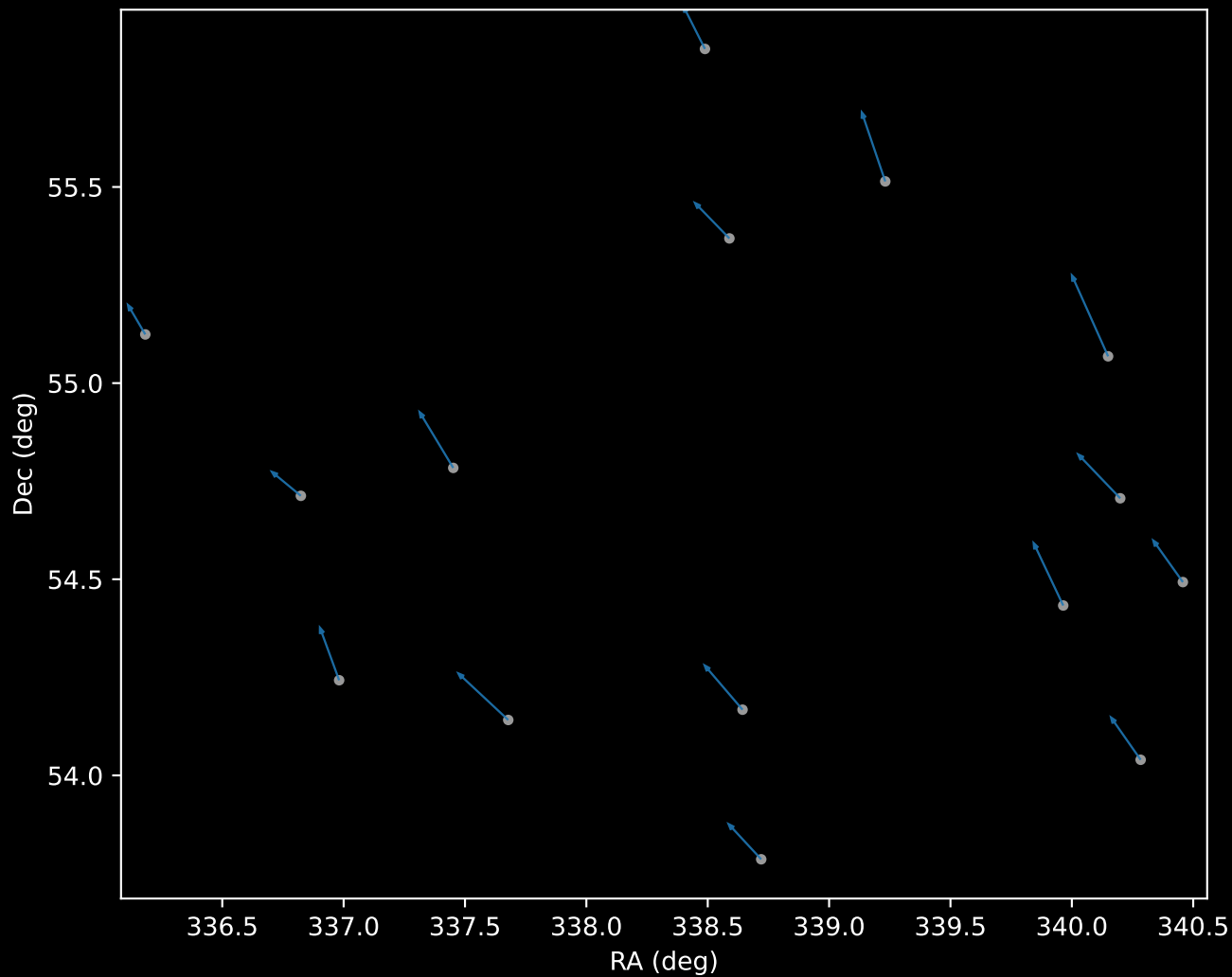
APOGEE DR17 Cluster 0 Proper Motion Vectors (n=15)
