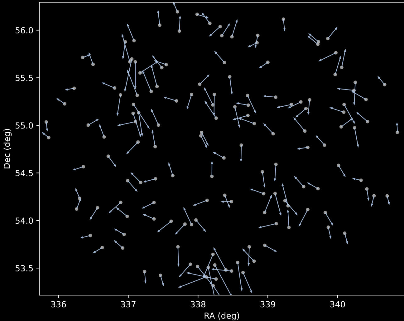
APOGEE DR17 Cluster 1 Proper Motion Vectors (n=145)
