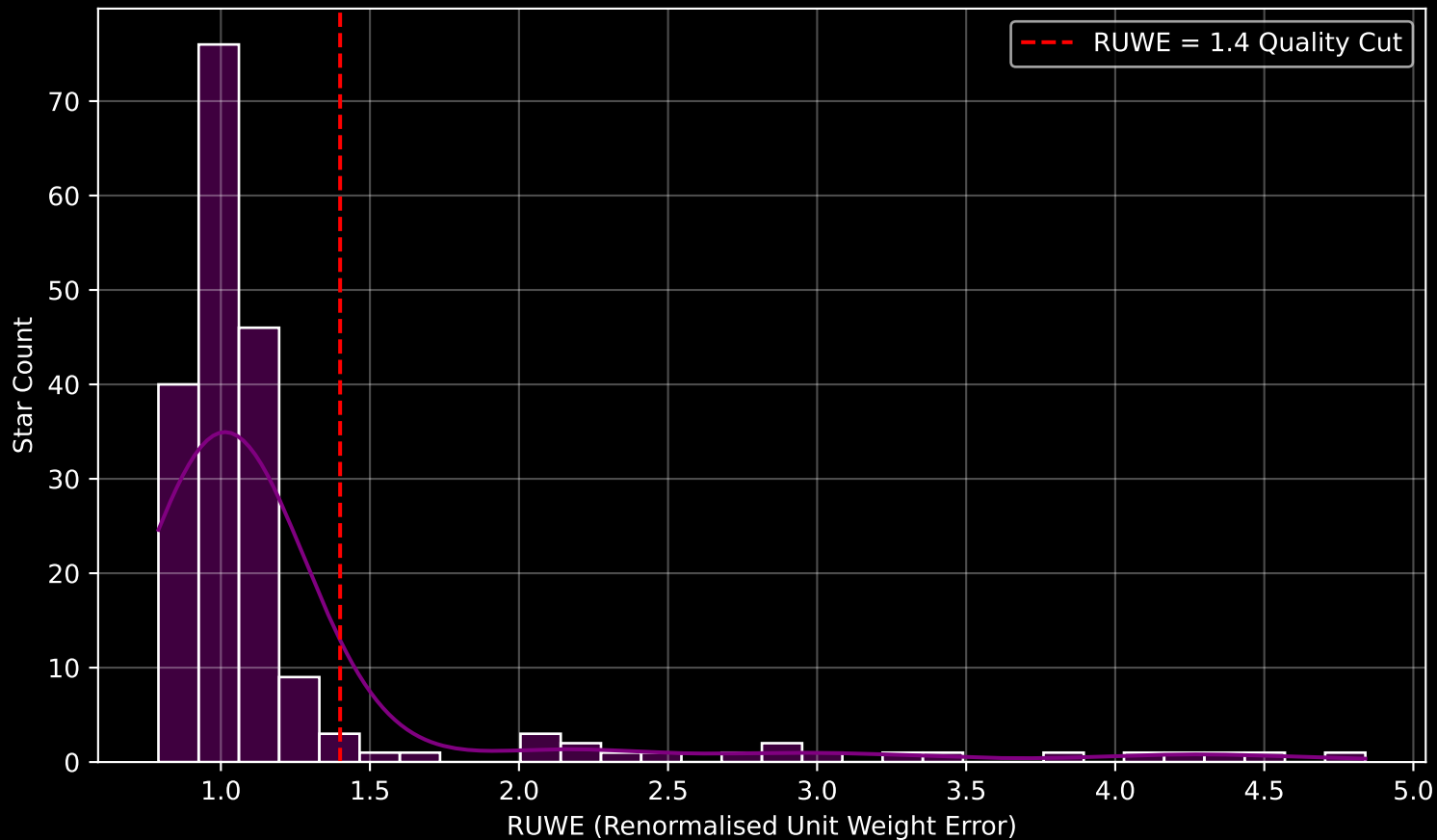
GAPOGEE DR17 Field [086+47_MGA] RUWE Distribution (n= 195)
